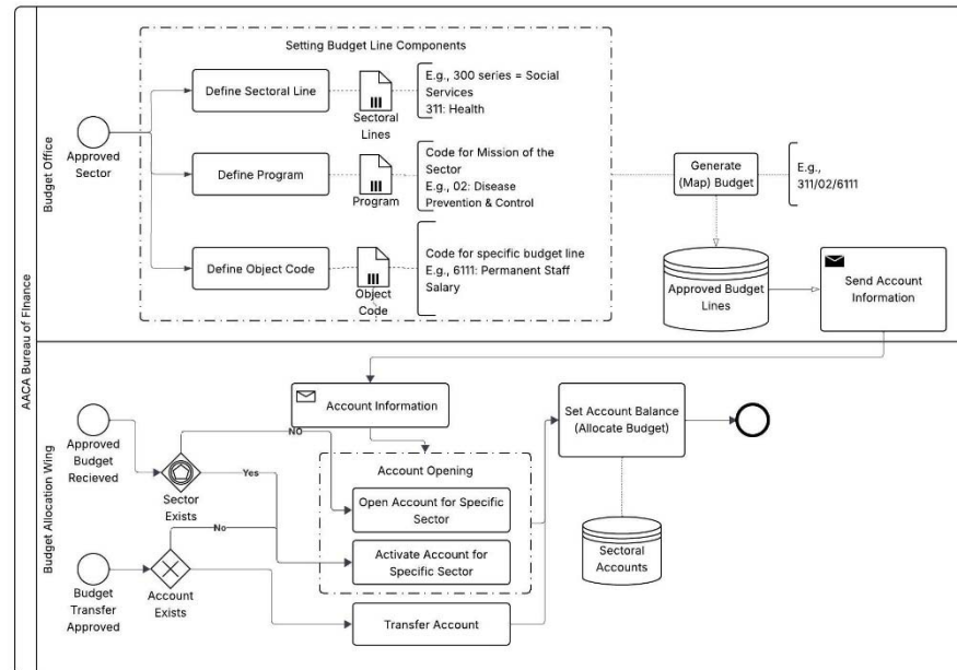
Figure 2-1: BPMN for Account Setting and Opening Balance
